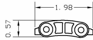
A1- SLAT NYLON RETAINER SECURED TO SLAT BY (2) #10X1 1/2" PFH SMS
