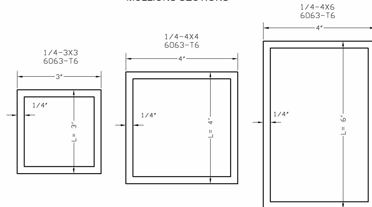
MULLIONS SECTIONS
